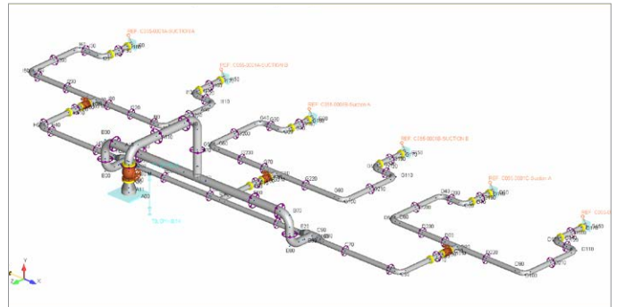
Determining the optimal arrangement for pipe supports automatically using Support Optimizer.
